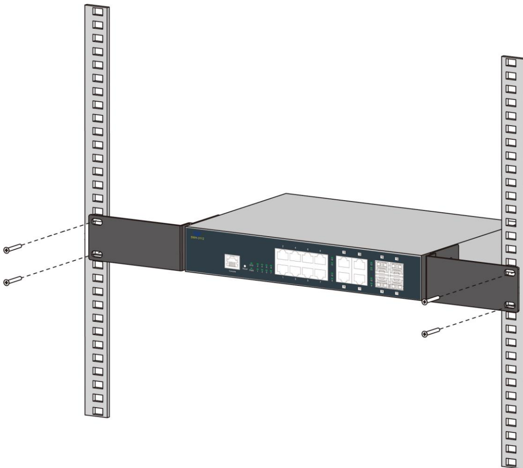
Figure 2-2. SWH-3112 Switch Rack-mounting
