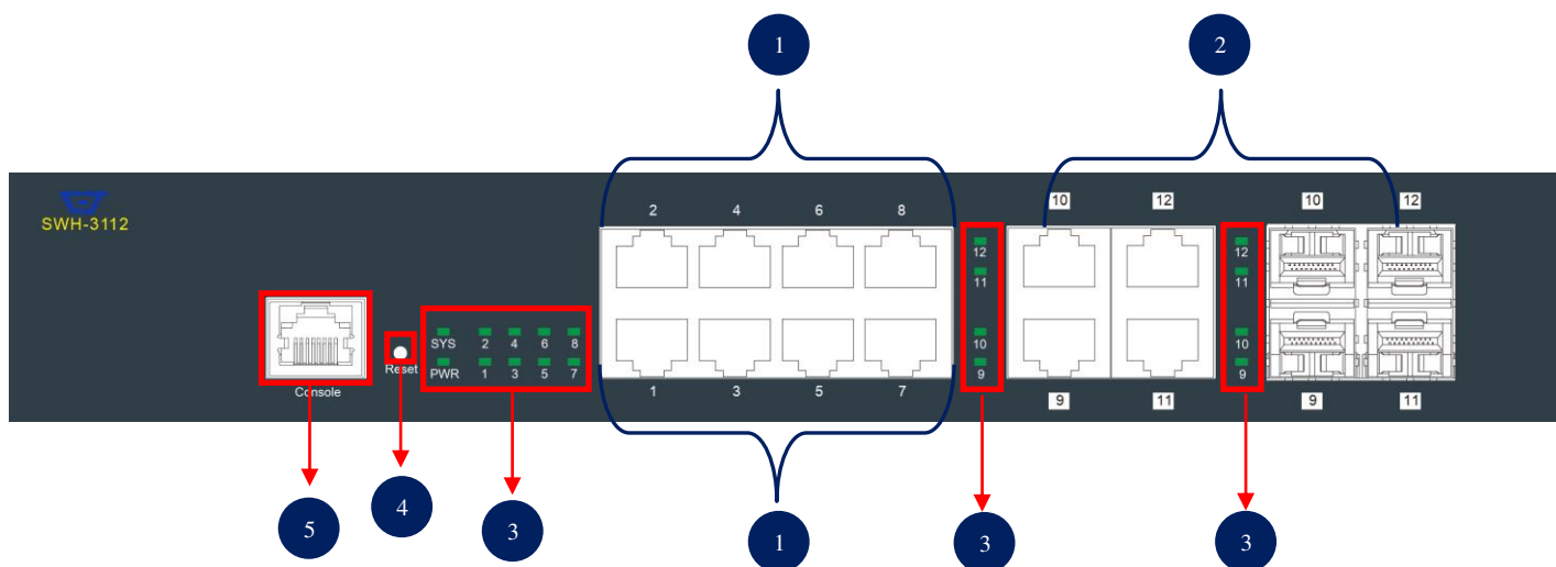
Figure 1-1. SWH-3112 Managed Switch Front Panel
