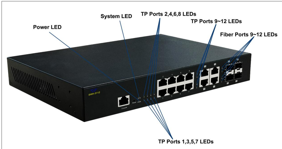
Figure 1-3. LEDs of SWH-3112 Managed Switch
