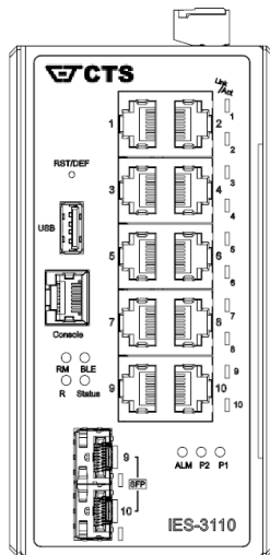
Figure 6. Install the Managed Industrial Gigabit Ethernet Switch in vertical direction.
