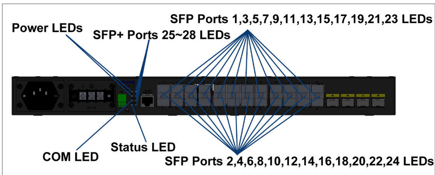
Figure 1-3. LEDs of FOS-5128 Managed Switch
