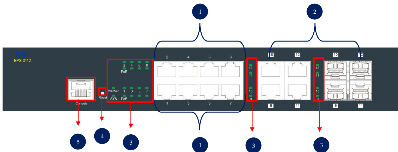
Figure 1-1. EPS-3112 Managed Switch Front Panel
